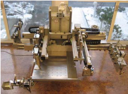
POLAR Restacking Station PickStack
