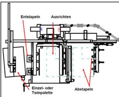
Layout of the PickStack
